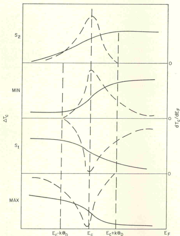
FIG. 9. Energy dependences of \Delta T_c (solid line) and \partial T_c / \partial E_F (broken line) as E_F passes through a critical point in the E(\mathbf{k}) spectrum. S_1 , S_2 , min., and max. refer to the critical points illustrated in Fig. 8.
